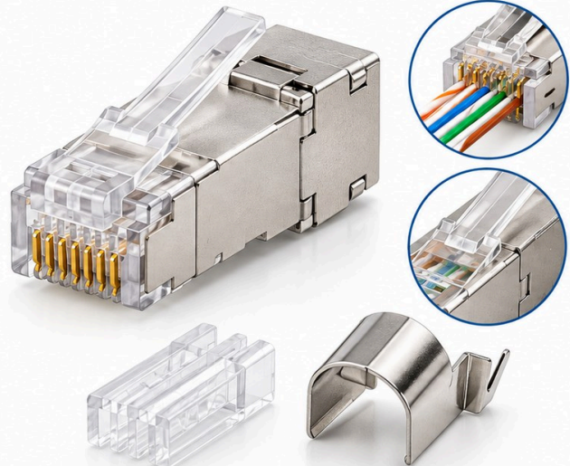
RJ45 Cat7 S/FTP Connector (EZ Pass-through)
